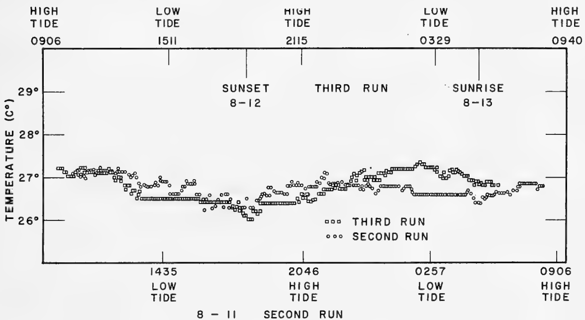
Figure 5. Temperature records for second and third runs, Buoy 1, at 170 ft.
